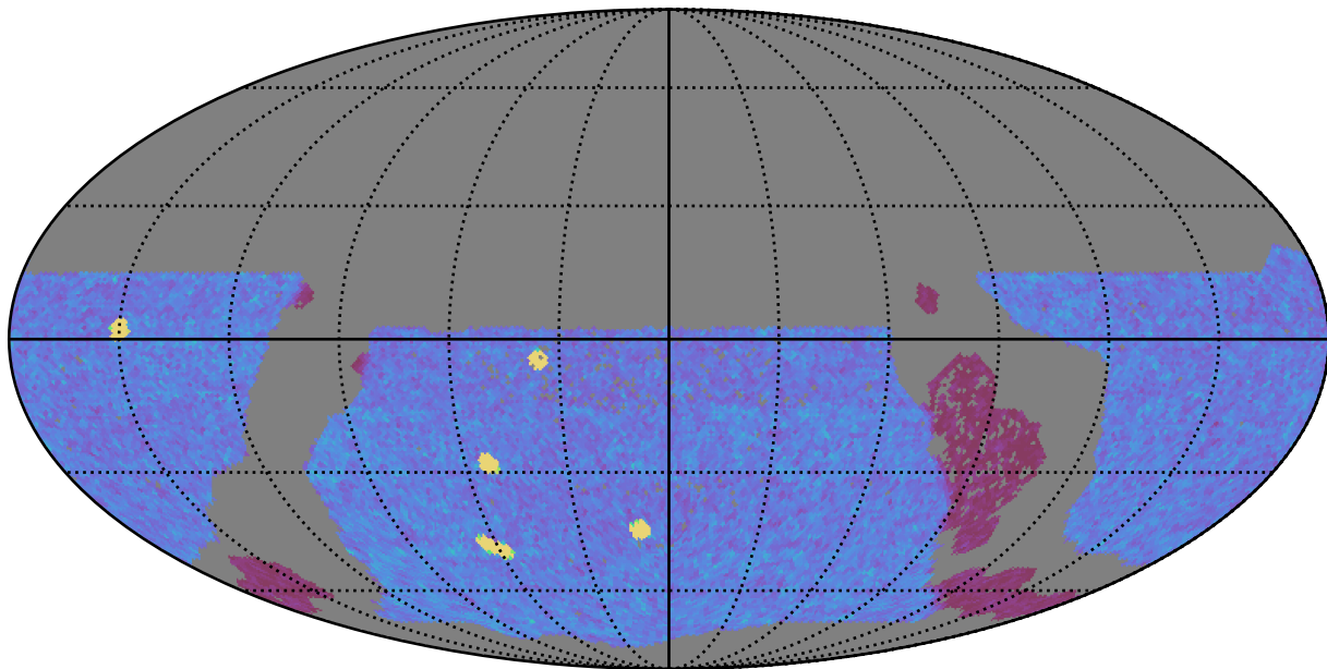
ddf_acor_sf10_lsf15_lsr10_v3.4_10yrs WFD y band: NVisits
