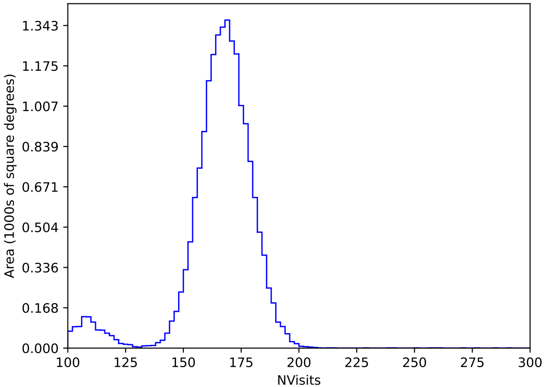
ddf_acor_sf10_lsf15_lsr10_v3.4_10yrs WFD y band: NVisits
