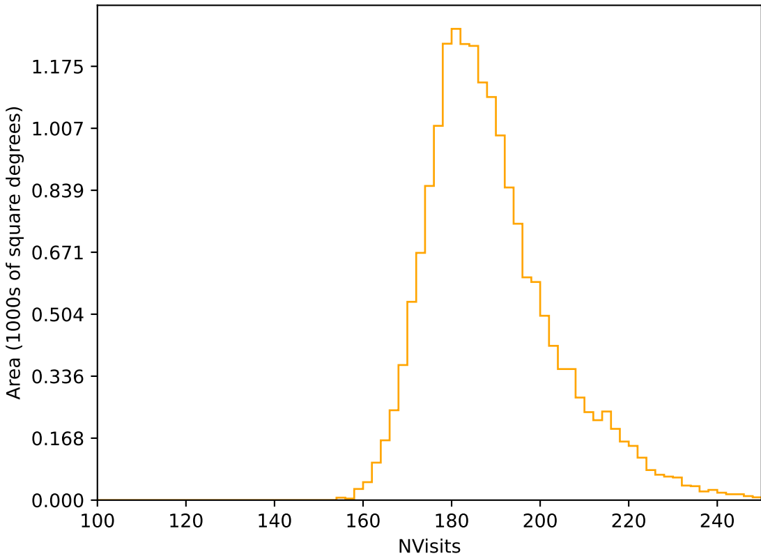
ddf_acor_sf10_lsf15_lsr10_v3.4_10yrs WFD r band: NVisits
