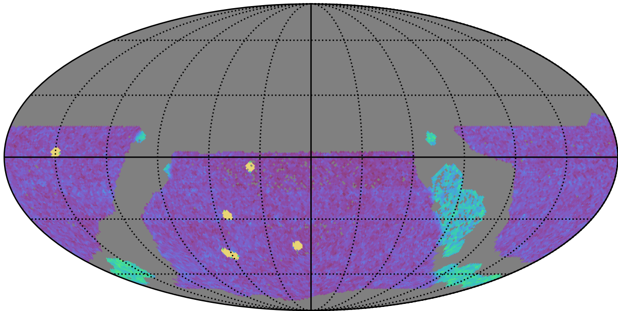
ddf_acor_sf10_lsf15_lsr10_v3.4_10yrs WFD g band: NVisits
