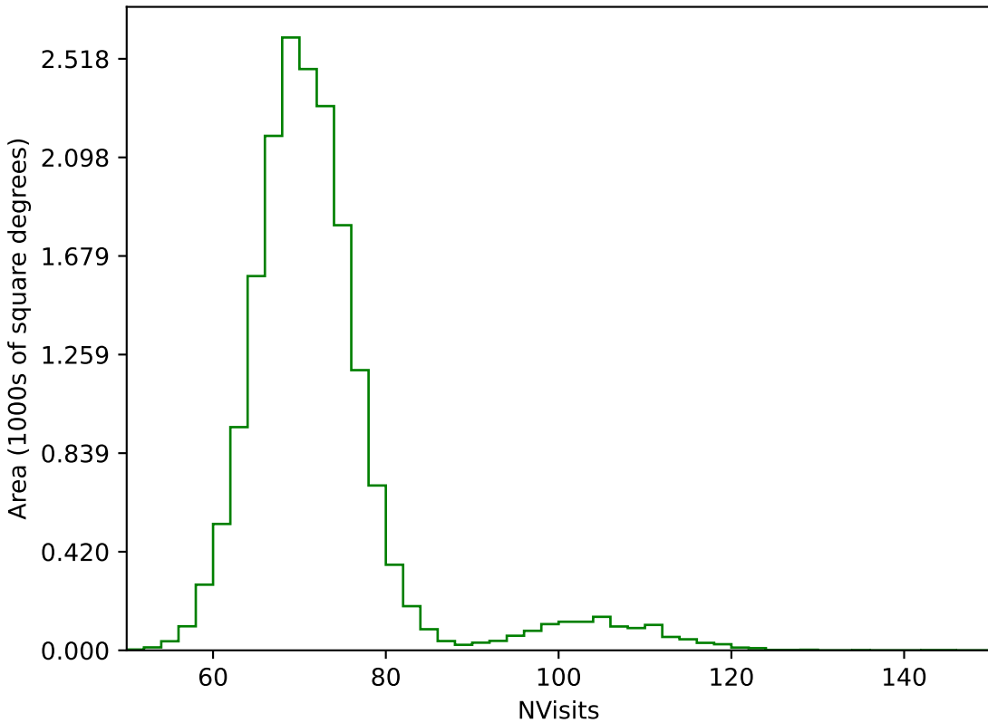
ddf_acor_sf10_lsf15_lsr10_v3.4_10yrs WFD g band: NVisits
