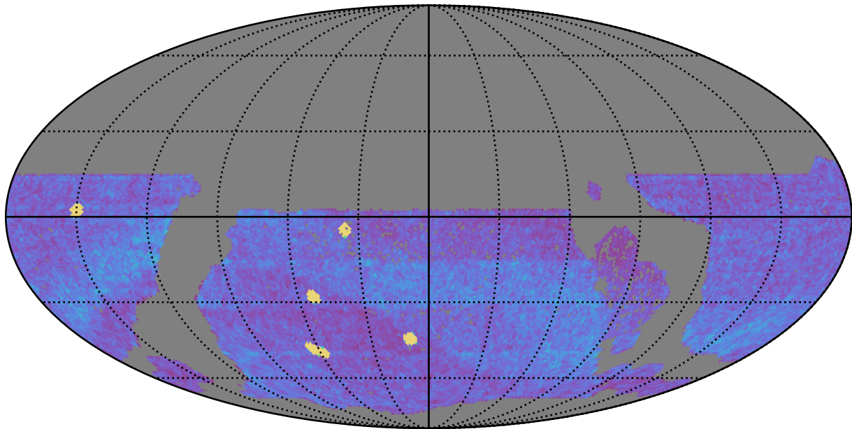
ddf_acor_sf10_lsf15_lsr10_v3.4_10yrs WFD all bands: NVisits
