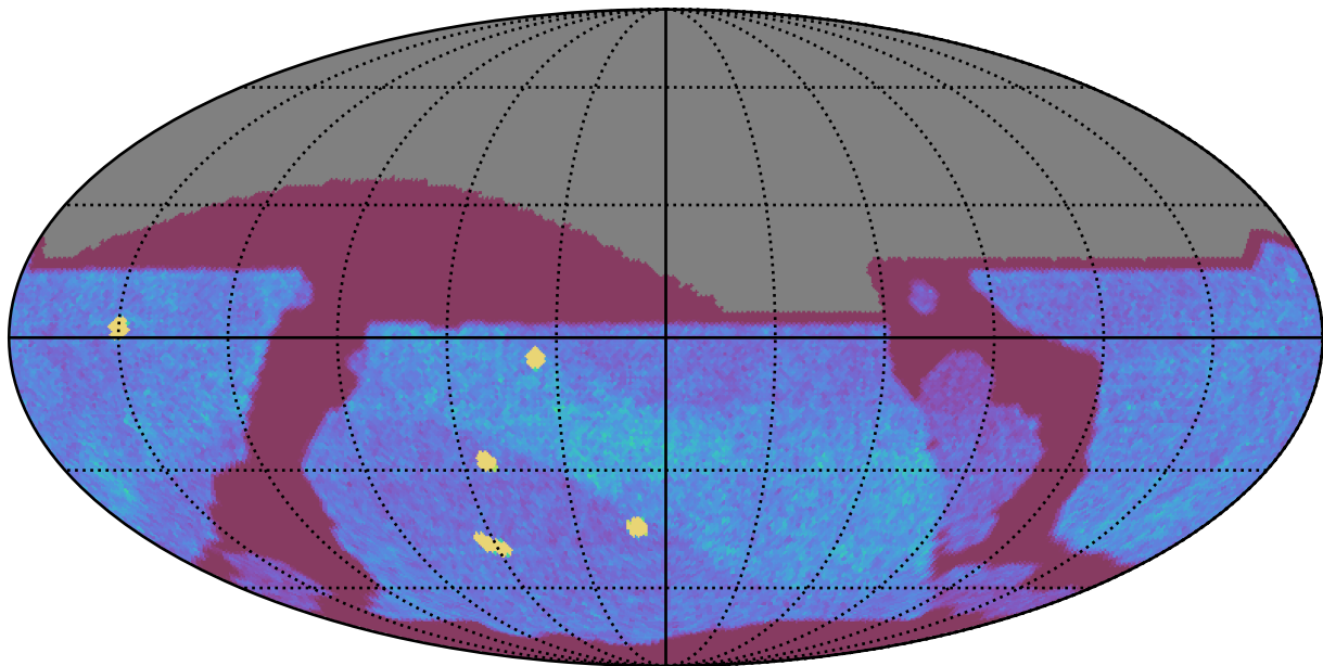
ddf_acor_sf10_lsf15_lsr10_v3.4_10yrs All sky z band: NVisits
