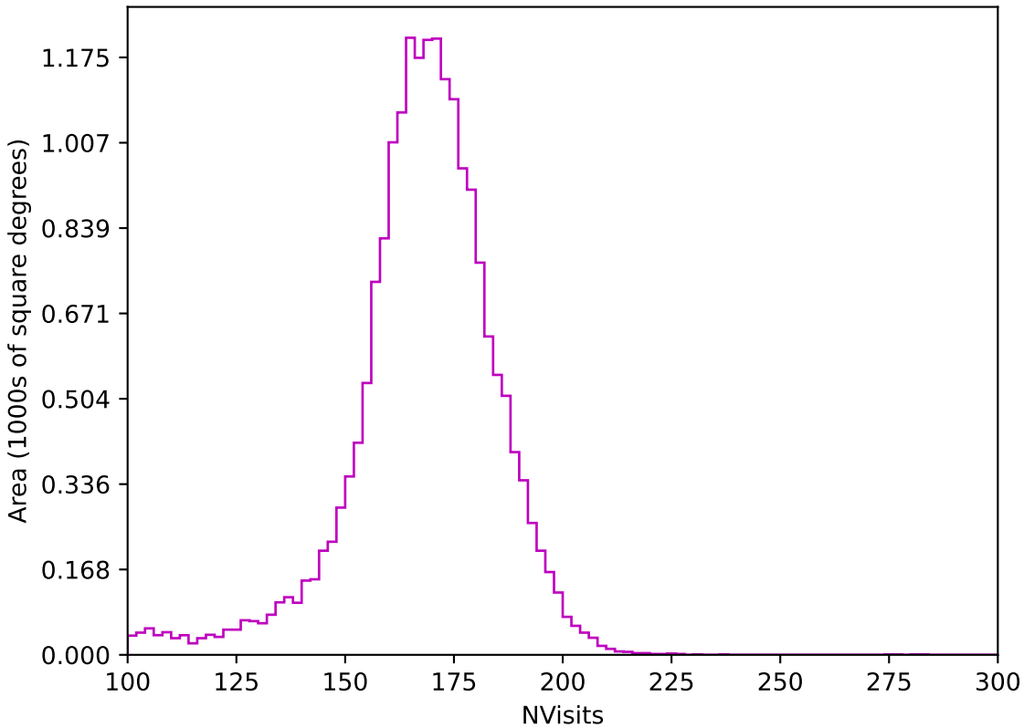
ddf_acor_sf10_ls15_lsr10_v3.4_10yrs All sky z band: NVisits
