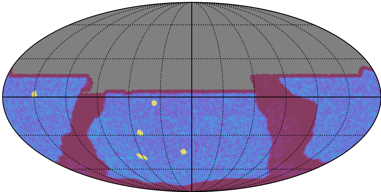
ddf_acor_sf10_lsf15_lsr10_v3.4_10yrs All sky y band: NVisits
