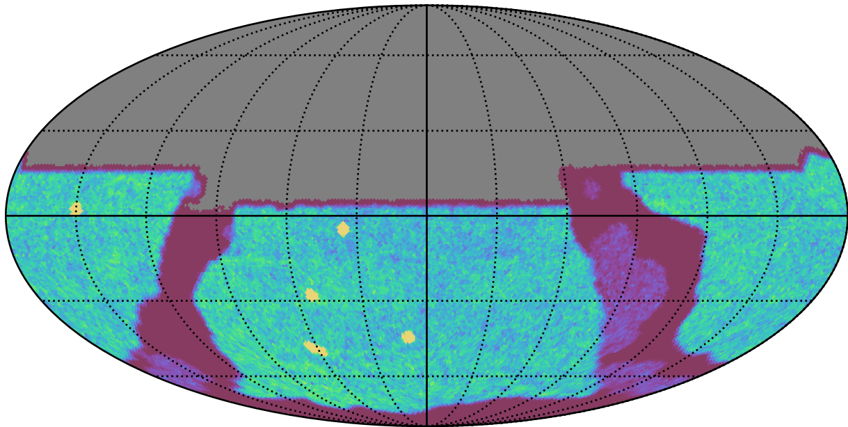
ddf_acor_sf10_lsf15_lsr10_v3.4_10yrs All sky u band: NVisits
