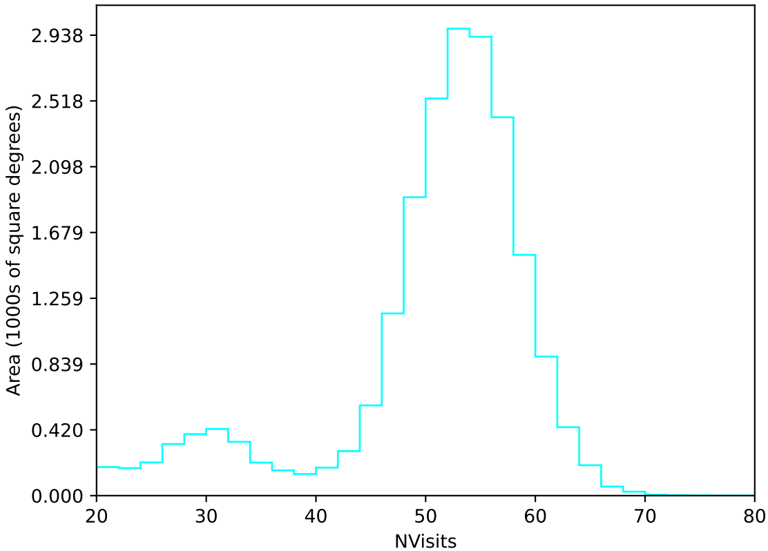
ddf_acor_sf10_ls15_lsr10_v3.4_10yrs All sky u band: NVisits
