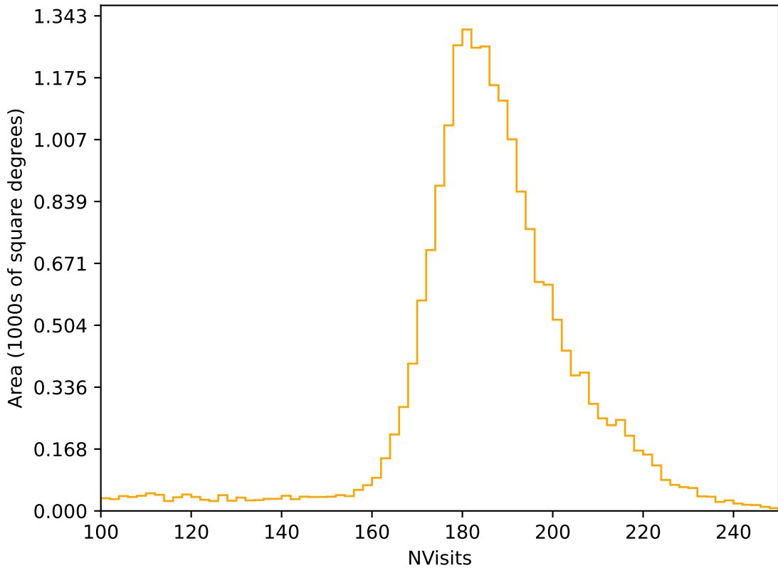
ddf_acor_sf10_lsf15_lsr10_v3.4_10yrs All sky r band: NVisits
