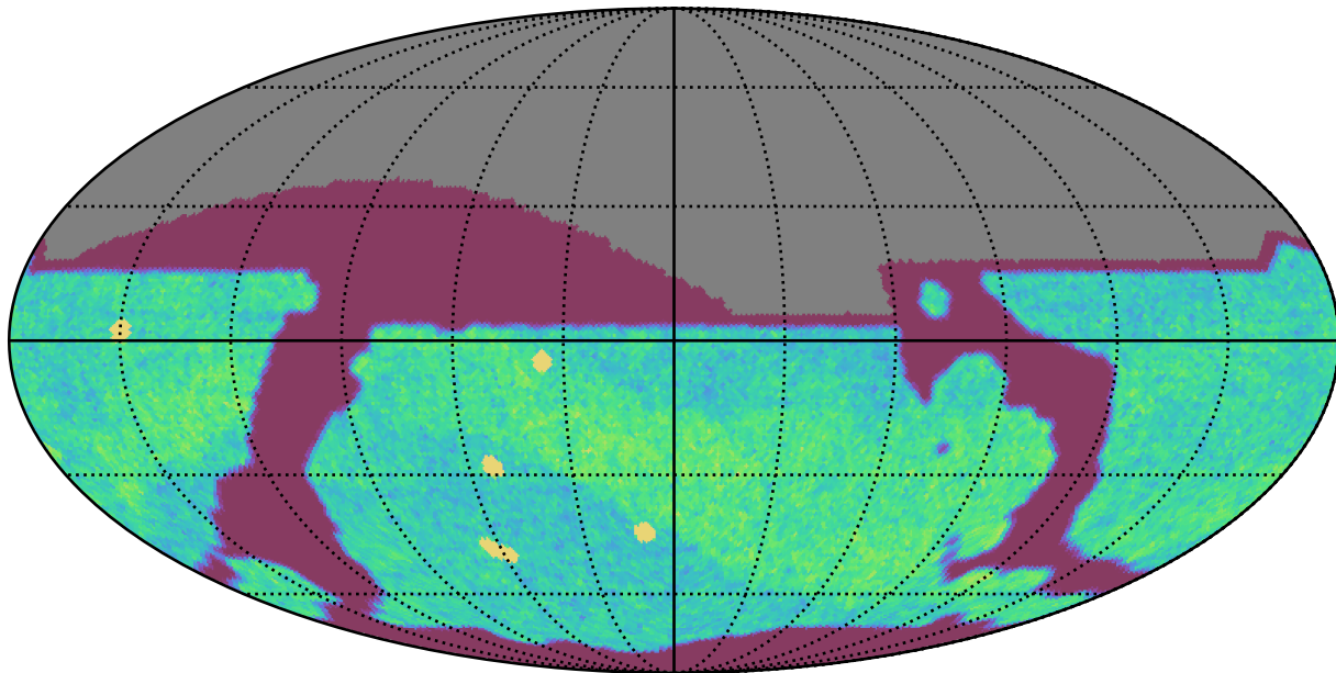
ddf_acor_sf10_lsf15_lsr10_v3.4_10yrs All sky i band: NVisits
