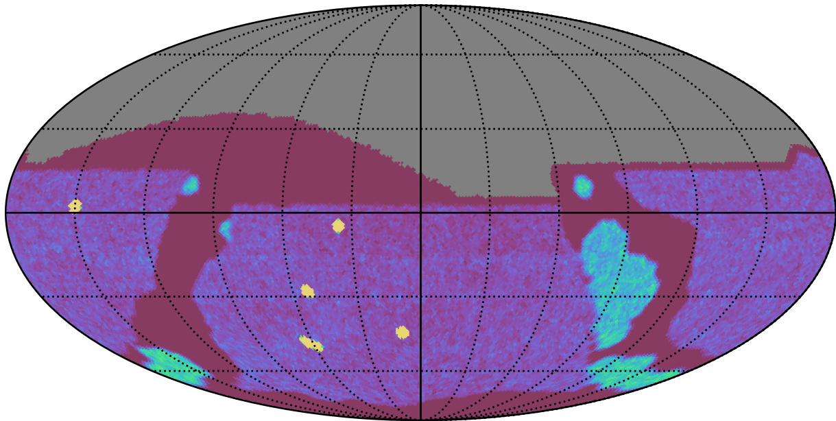
ddf_acor_sf10_lsf15_lsr10_v3.4_10yrs All sky g band: NVisits
