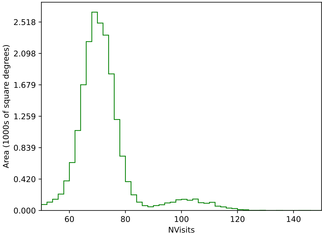
ddf_acor_sf10_lsf15_lsr10_v3.4_10yrs All sky g band: NVisits
