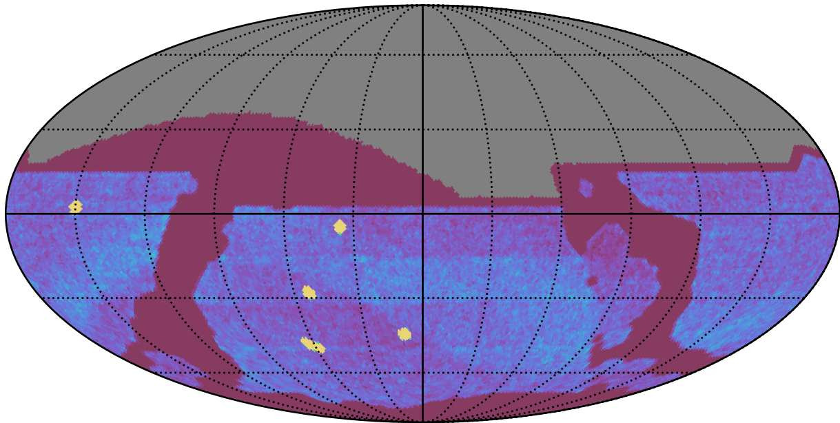
ddf_acor_sf10_lsf15_lsr10_v3.4_10yrs All sky all bands: NVisits
