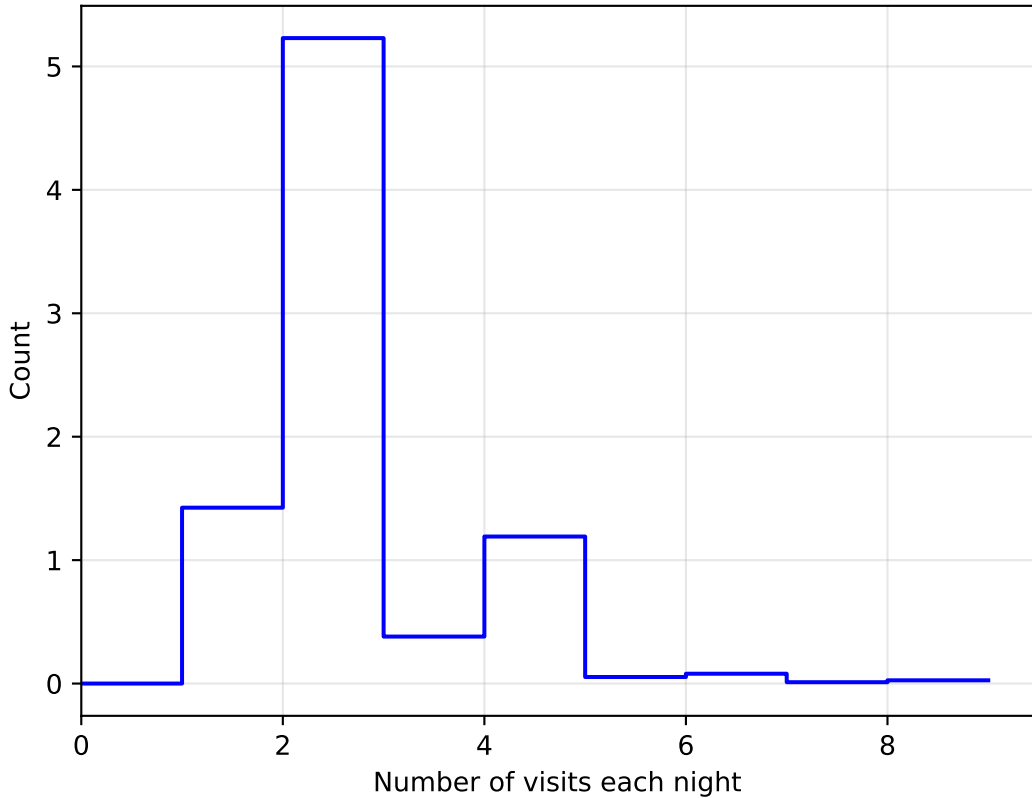
ddf_acor_sf10_lsf15_lsr10_v3.4_10yrs WFD: NVisitsPerNight 1e6
