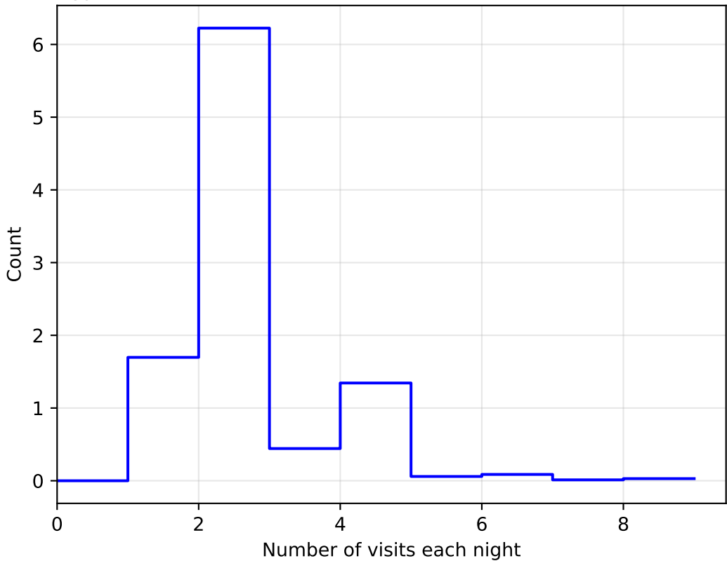
ddf_acor_sf10_lsf15_lsr10_v3.4_10yrs All sky: NVisitsPerNight 1e6
