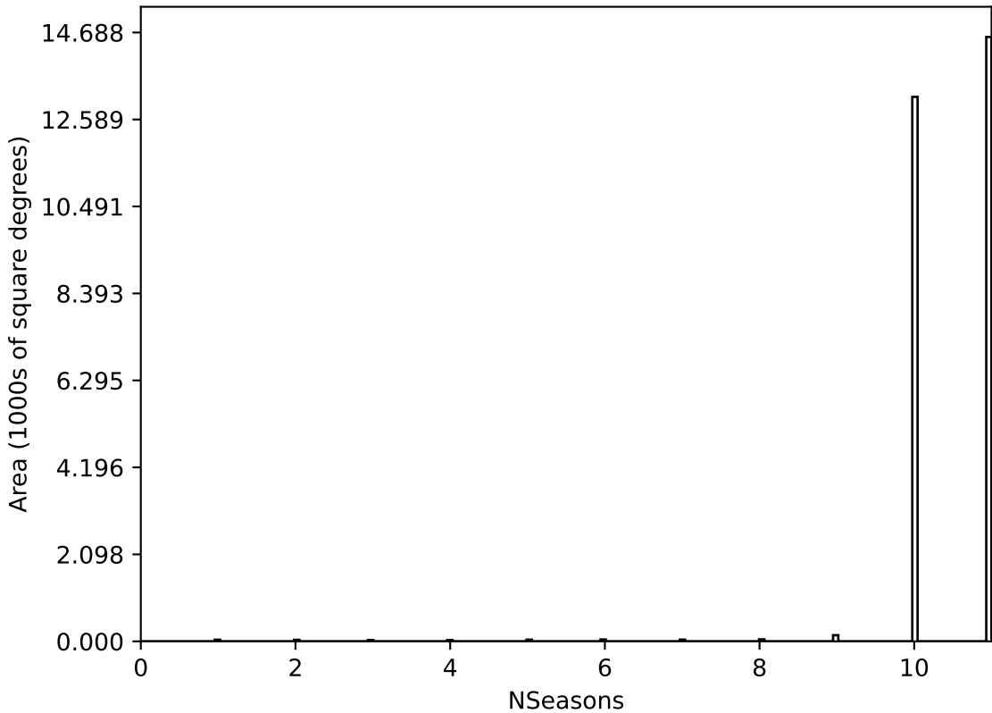
ddf_acor_sf10_lsf15_lsr10_v3.4_10yrs All sky all bands: NSeasons
