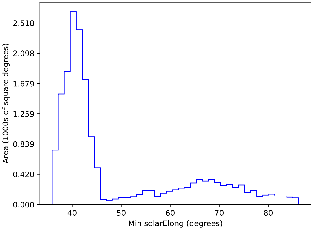
ddf_acor_sf10_lsf15_lsr10_v3.4_10yrs WFD z band: Min solarElong
