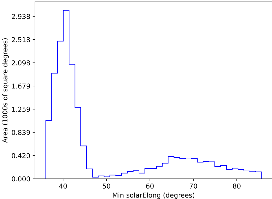
ddf_acor_sf10_lsf15_lsr10_v3.4_10yrs WFD i band: Min solarElong
