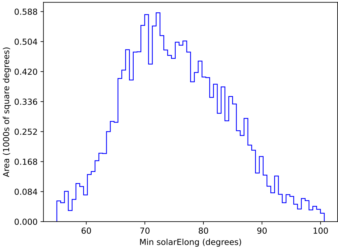
ddf_acor_sf10_lsf15_lsr10_v3.4_10yrs WFD g band: Min solarElong
