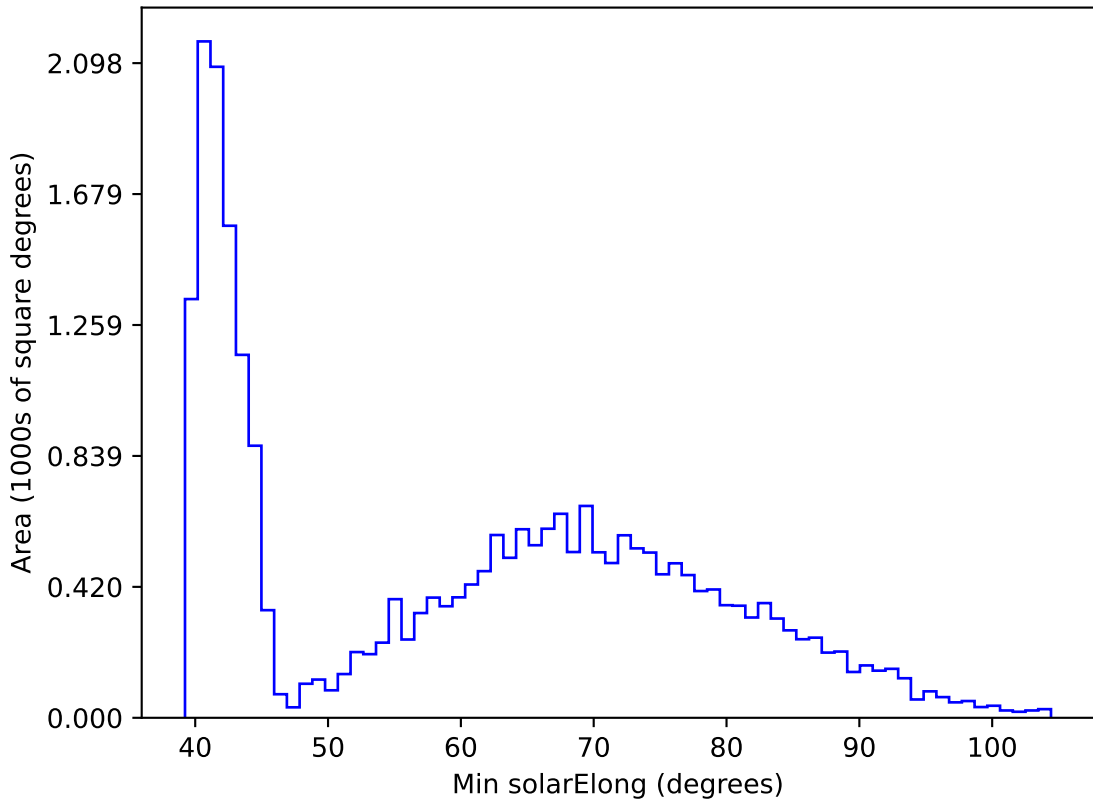
ddf_acor_sf10_ls15_lsr10_v3.4_10yrs All sky r band: Min solarElong
