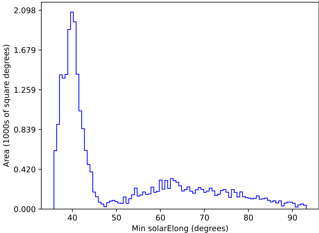
ddf_acor_sf10_lsf15_lsr10_v3.4_10yrs All sky all bands: Min solarElong
