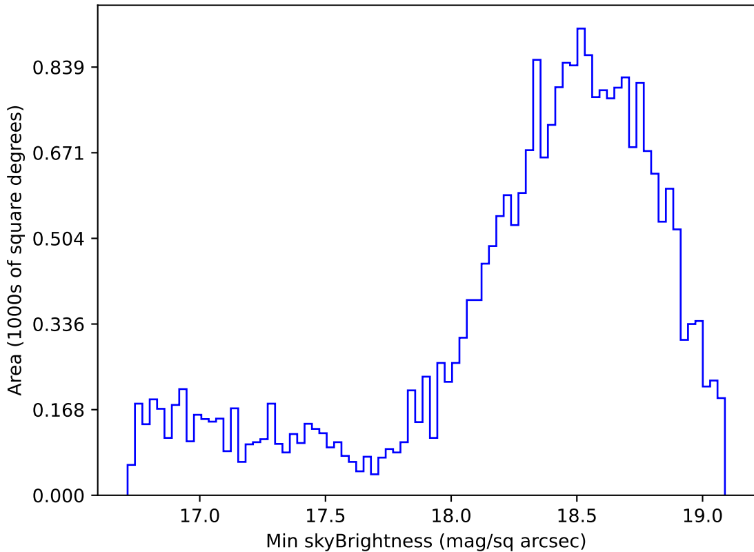
ddf_acor_sf10_lsf15_lsr10_v3.4_10yrs Yr 1 z band: Min skyBrightness
