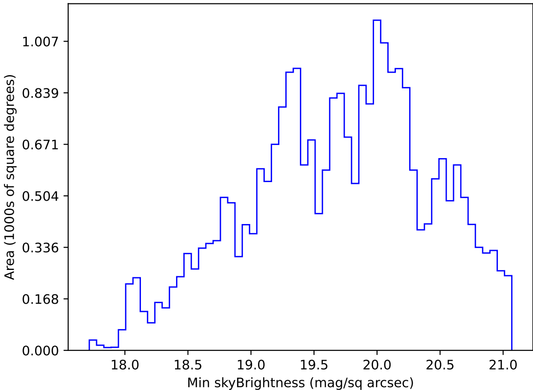
ddf_acor_sf10_lsf15_lsr10_v3.4_10yrs Yr 1 r band: Min skyBrightness
