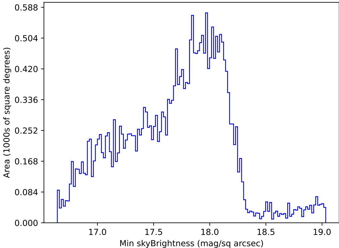
ddf_acor_sf10_lsf15_lsr10_v3.4_10yrs Yr 1 all bands: Min skyBrightness
