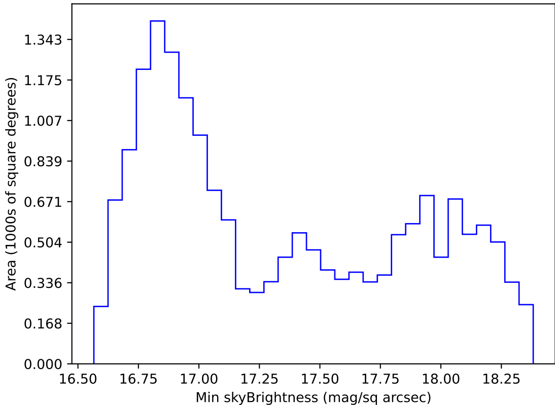
ddf_acor_sf10_lsf15_lsr10_v3.4_10yrs WFD z band: Min skyBrightness
