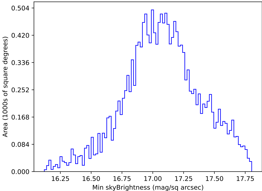
ddf_acor_sf10_lsf15_lsr10_v3.4_10yrs WFD y band: Min skyBrightness
