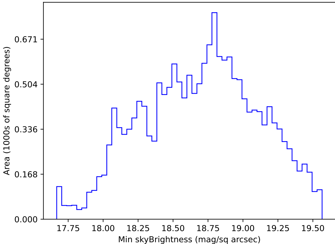
ddf_acor_sf10_lsf15_lsr10_v3.4_10yrs WFD r band: Min skyBrightness
