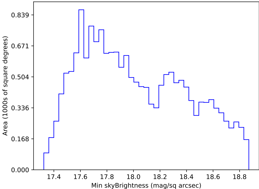
ddf_acor_sf10_lsf15_lsr10_v3.4_10yrs WFD i band: Min skyBrightness
