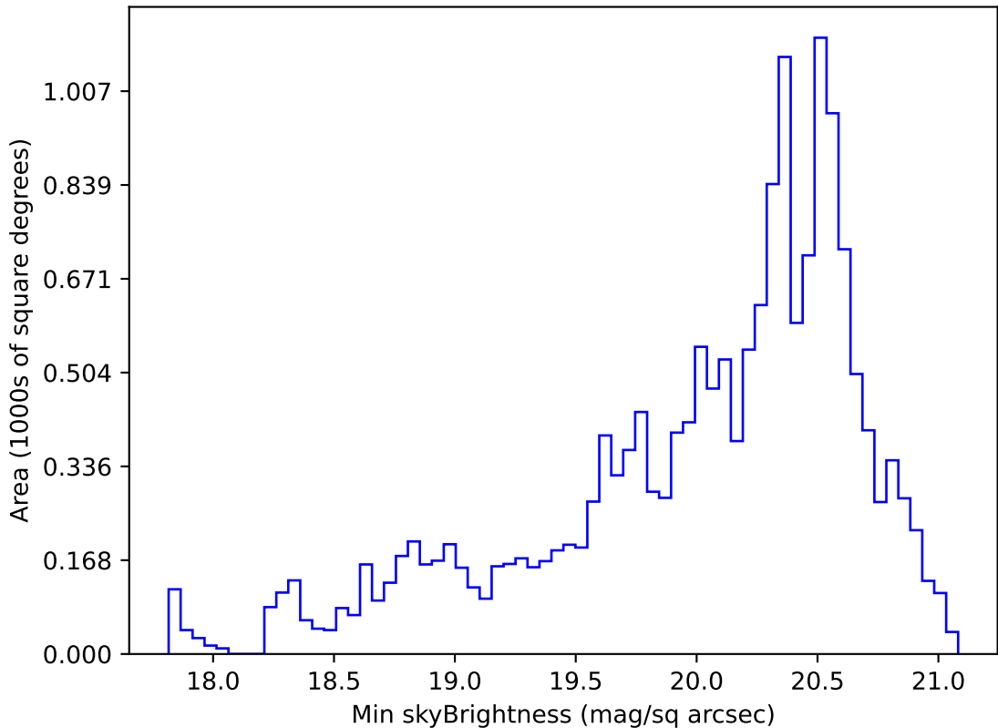
ddf_acor_sf10_lsf15_lsr10_v3.4_10yrs WFD g band: Min skyBrightness
