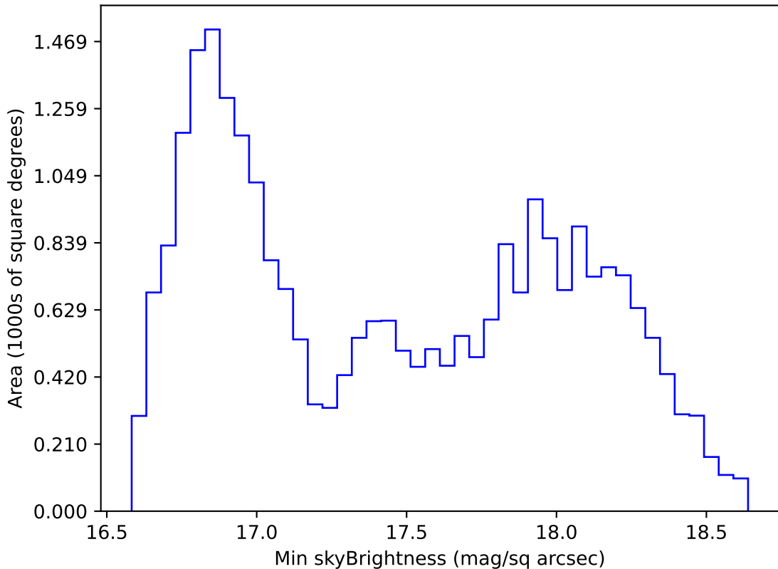
ddf_acor_sf10_lsf15_lsr10_v3.4_10yrs All sky z band: Min skyBrightness
