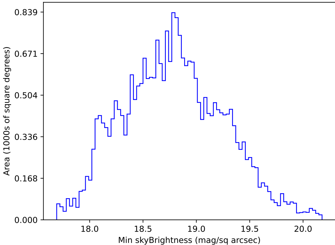
ddf_acor_sf10_lsf15_lsr10_v3.4_10yrs All sky r band: Min skyBrightness
