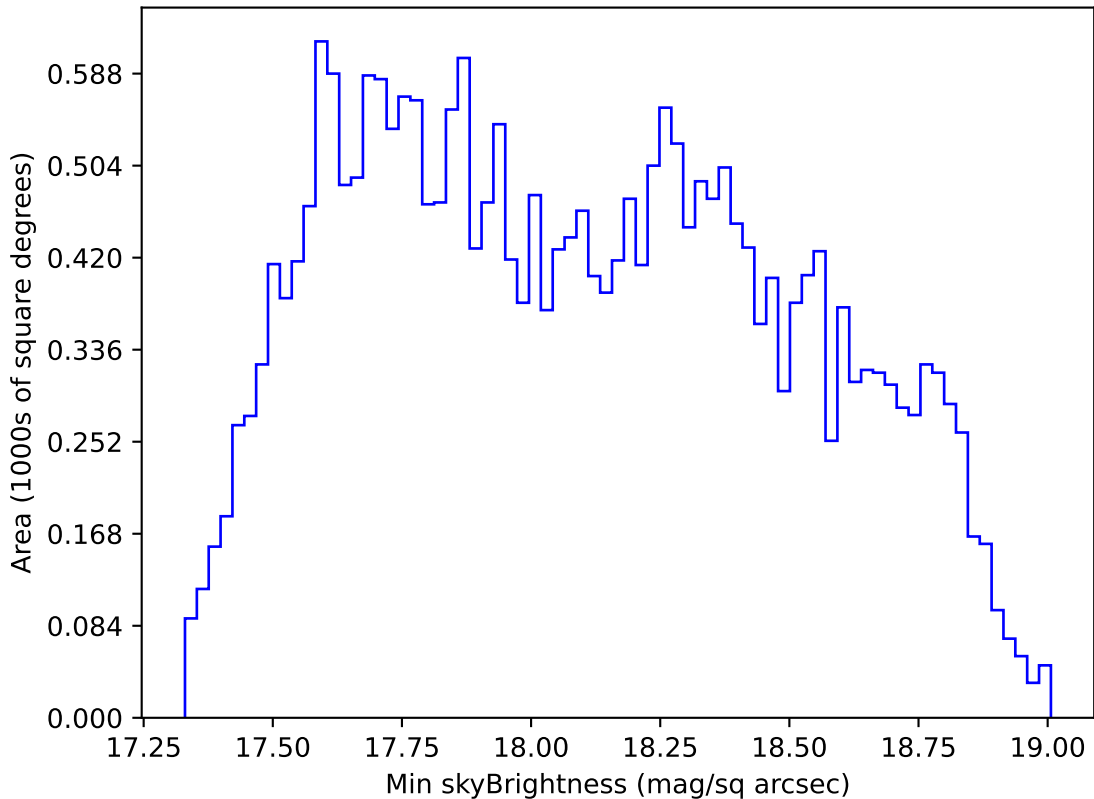
ddf_acor_sf10_lsf15_lsr10_v3.4_10yrs All sky i band: Min skyBrightness
