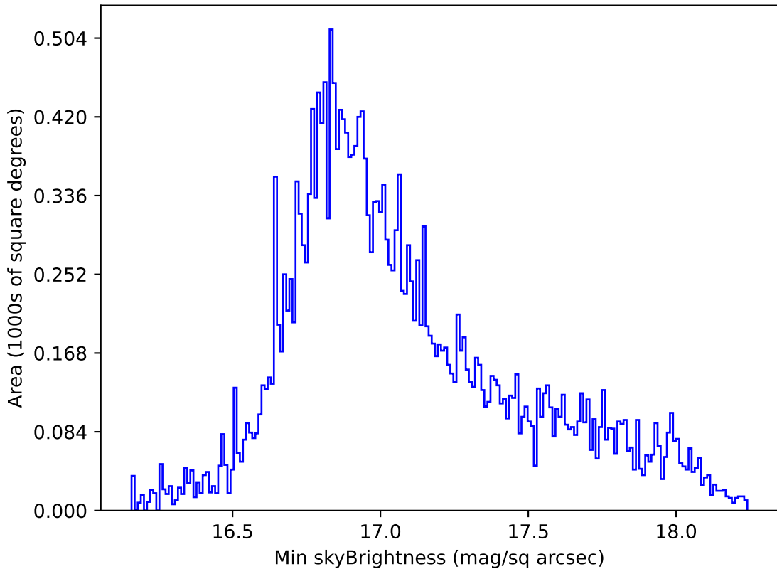
ddf_acor_sf10_lsf15_lsr10_v3.4_10yrs All sky all bands: Min skyBrightness
