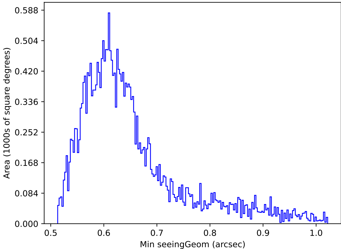
ddf_acor_sf10_ls15_lsr10_v3.4_10yrs Yr 1 z band: Min seeingGeom
