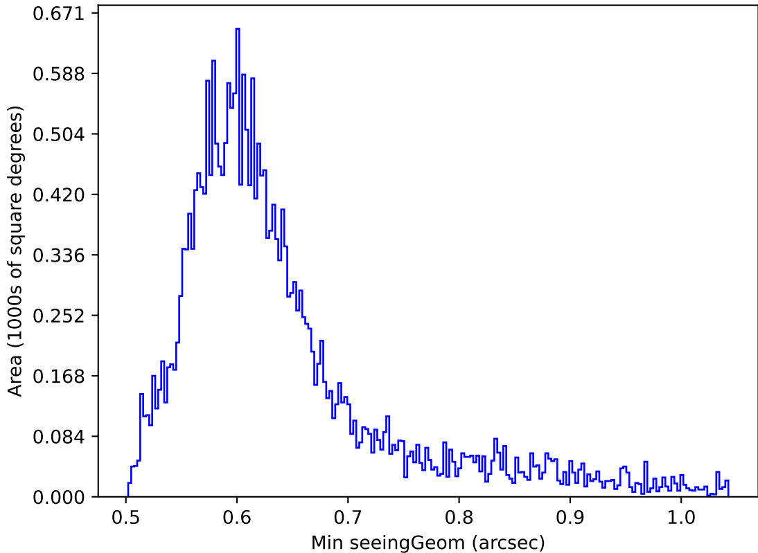
ddf_acor_sf10_lsf15_lsr10_v3.4_10yrs Yr 1 i band: Min seeingGeom
