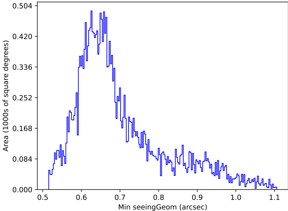
ddf_acor_sf10_ls15_lsr10_v3.4_10yrs Yr 1 g band: Min seeingGeom
