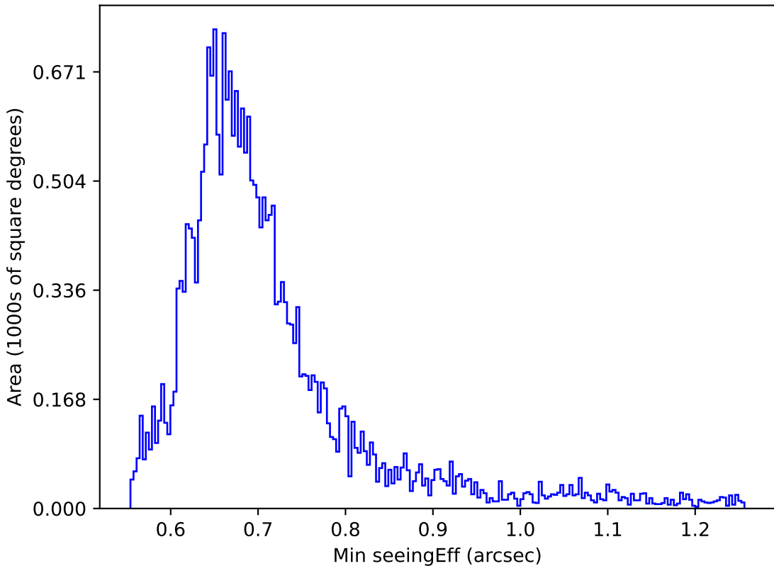
ddf_acor_sf10_ls15_lsr10_v3.4_10yrs Yr 1 r band: Min seeingEff
