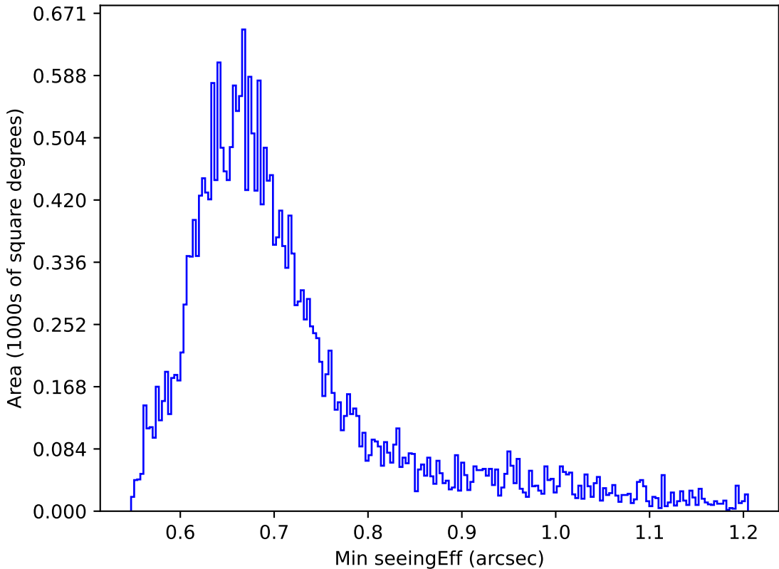
ddf_acor_sf10_lsf15_lsr10_v3.4_10yrs Yr 1 i band: Min seeingEff
