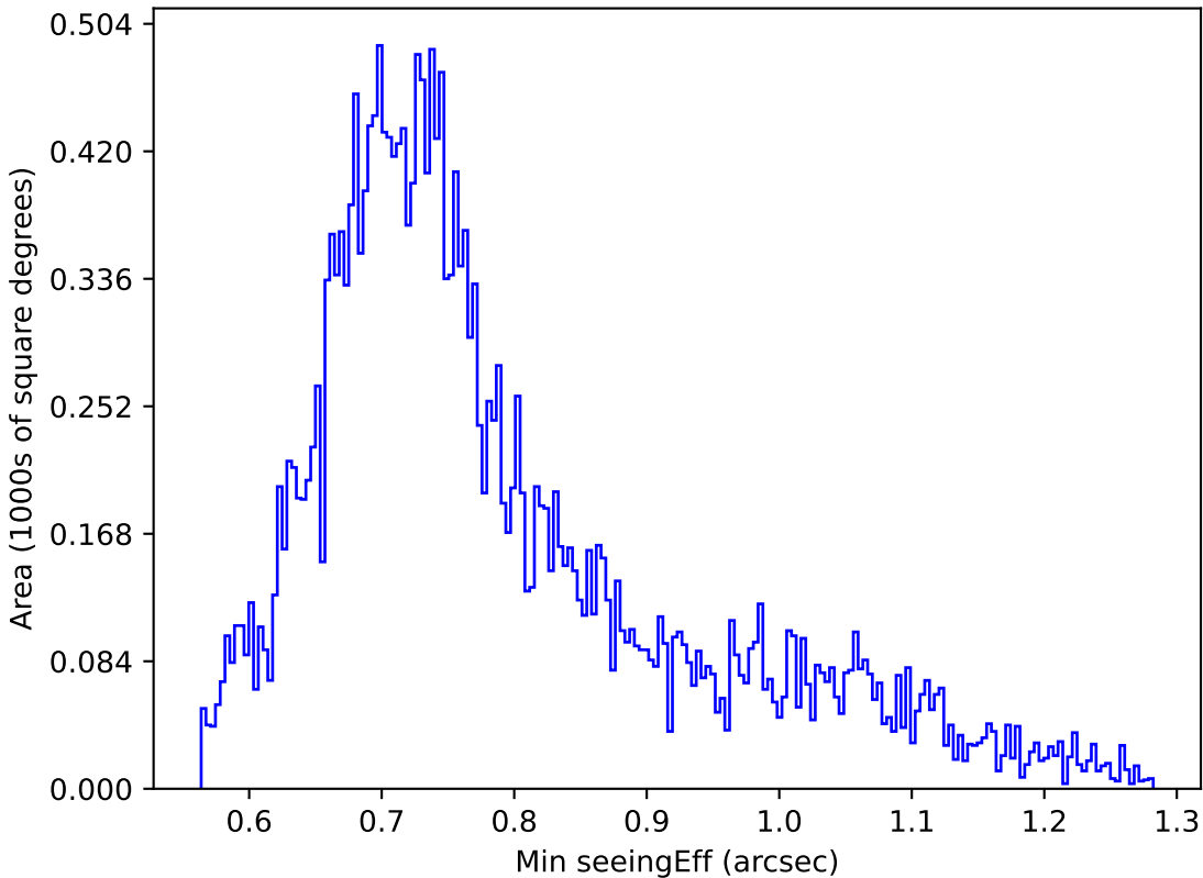
ddf_acor_sf10_ls15_lsr10_v3.4_10yrs Yr 1 g band: Min seeingEff
