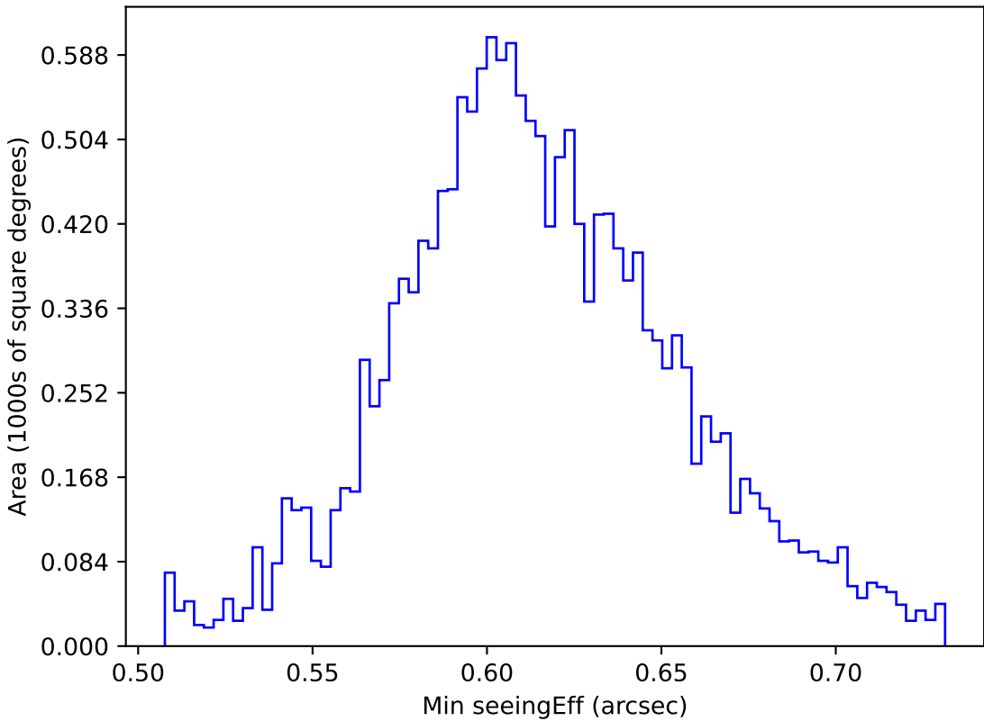
ddf_acor_sf10_lsf15_lsr10_v3.4_10yrs WFD z band: Min seeingEff
