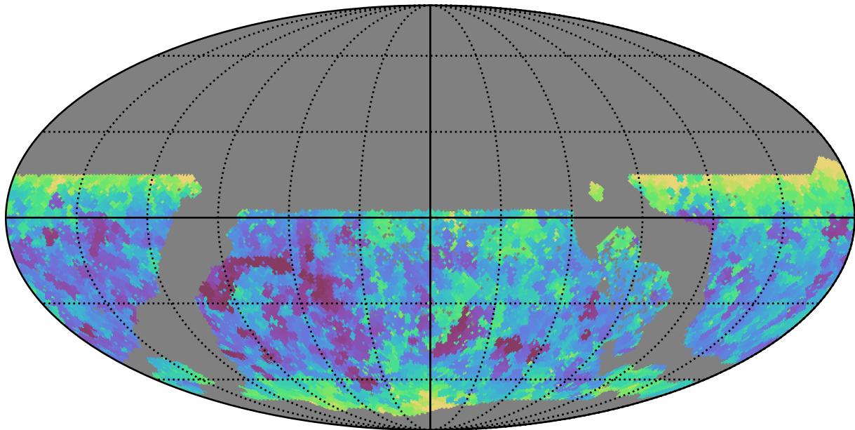
ddf_acor_sf10_lsf15_lsr10_v3.4_10yrs WFD y band: Min seeingEff
