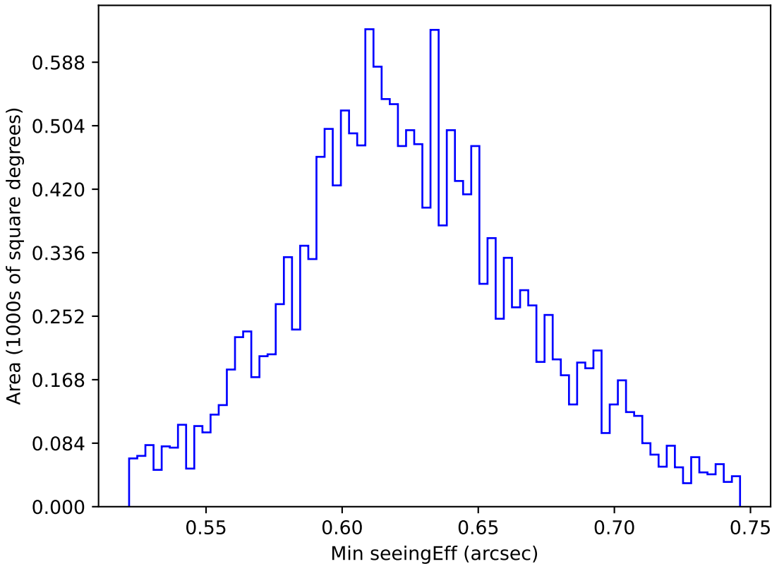
ddf_acor_sf10_lsf15_lsr10_v3.4_10yrs WFD y band: Min seeingEff
