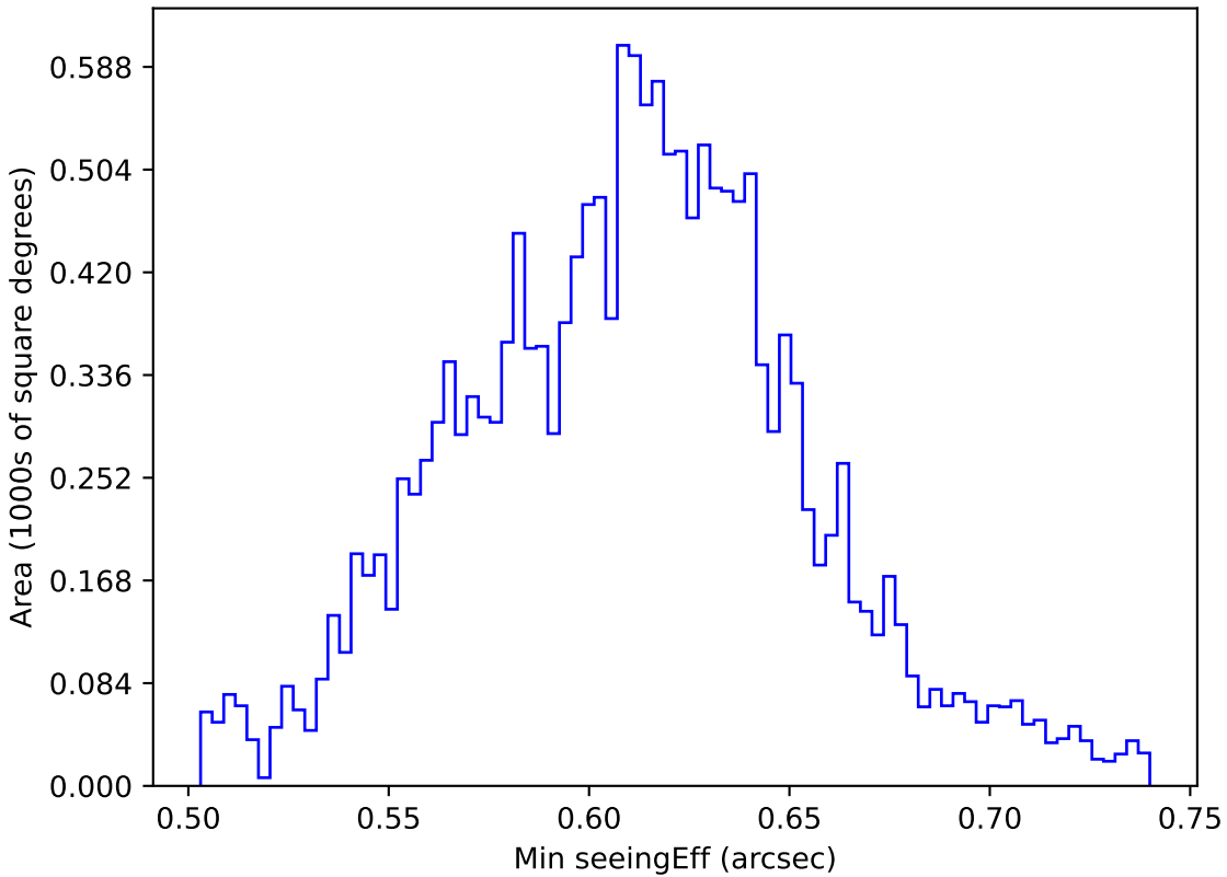
ddf_acor_sf10_lsf15_lsr10_v3.4_10yrs WFD r band: Min seeingEff
