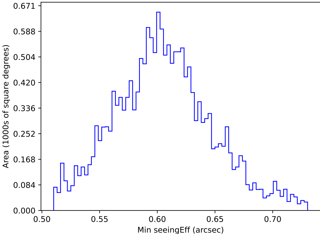
ddf_acor_sf10_lsf15_lsr10_v3.4_10yrs WFD i band: Min seeingEff
