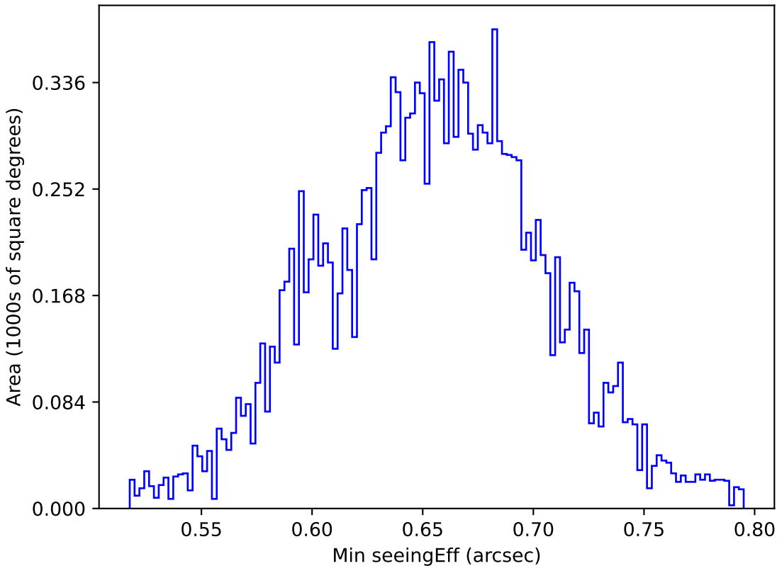
ddf_acor_sf10_lsf15_lsr10_v3.4_10yrs WFD g band: Min seeingEff
