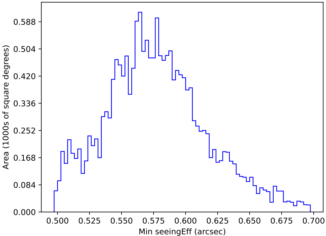
ddf_acor_sf10_ls15_lsr10_v3.4_10yrs WFD all bands: Min seeingEff
