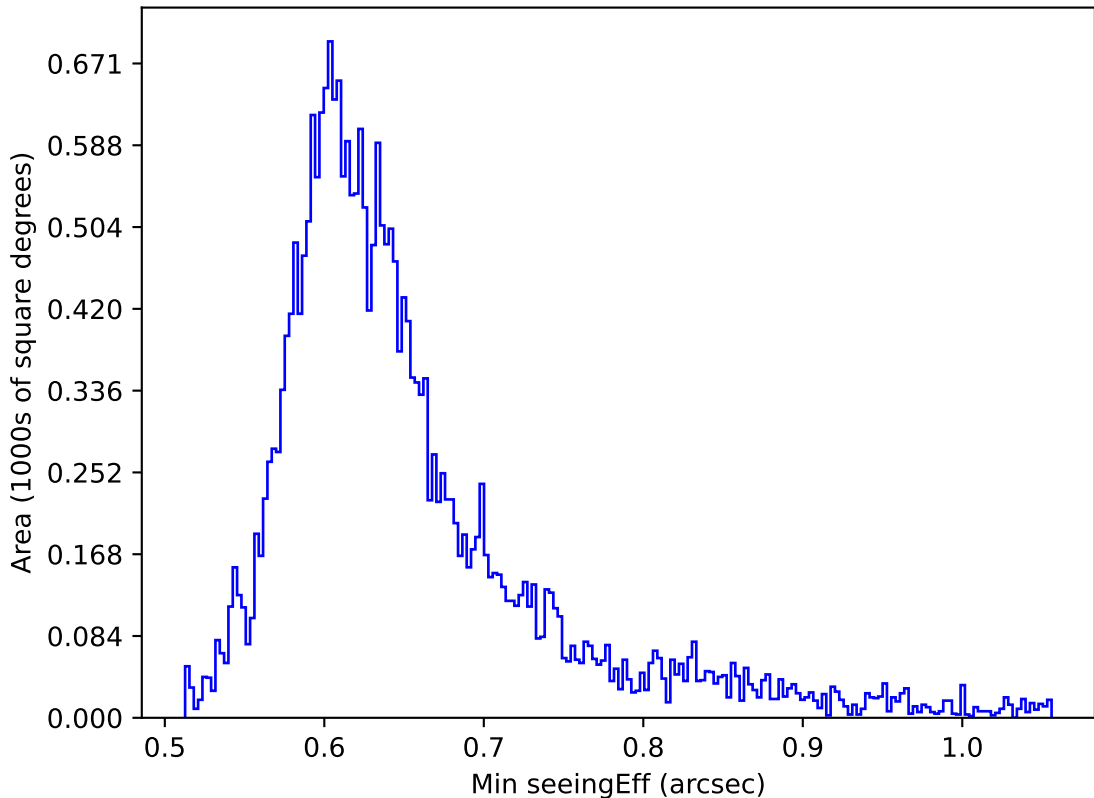
ddf_acor_sf10_lsf15_lsr10_v3.4_10yrs All sky z band: Min seeingEff
